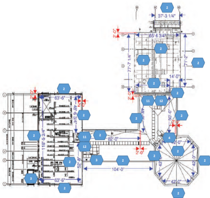
SECOND FLOOR PLAN 1/16" = 1'-0"
