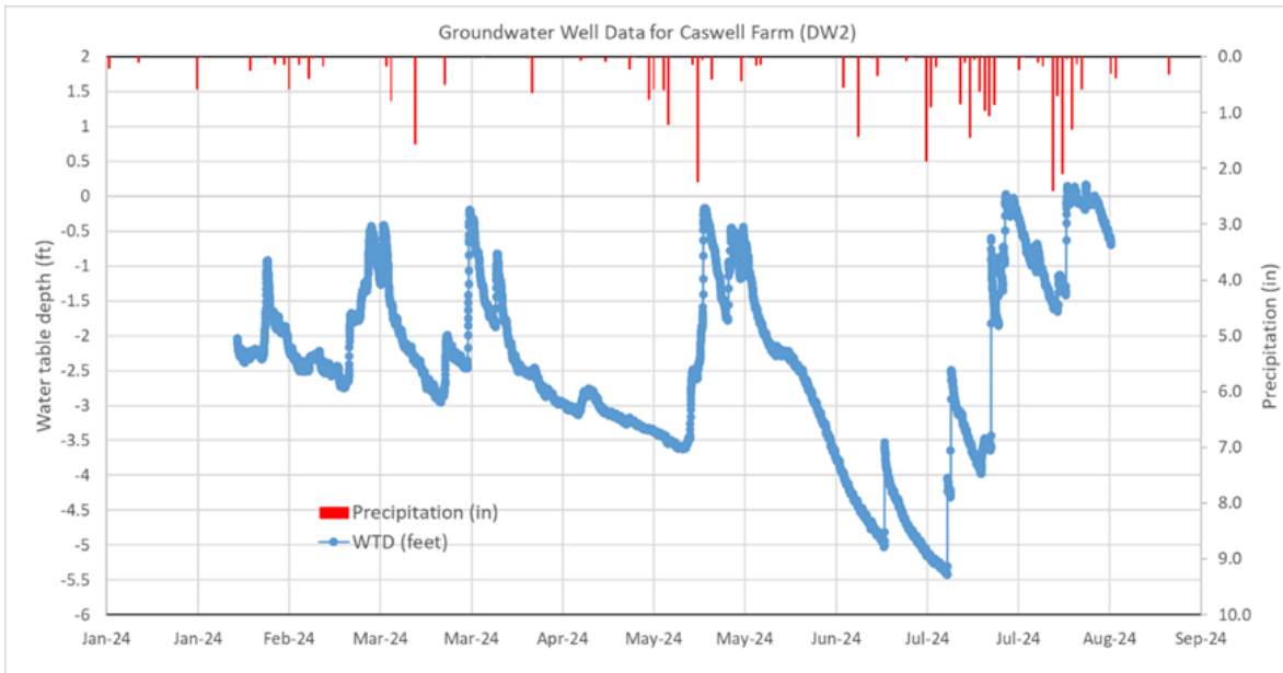
Figure 3. Groundwater Monitoring Data and Rainfall Depths for the Period
