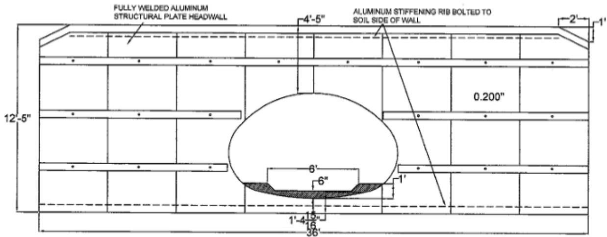
END VIEW- OUTLET HEADWALL
