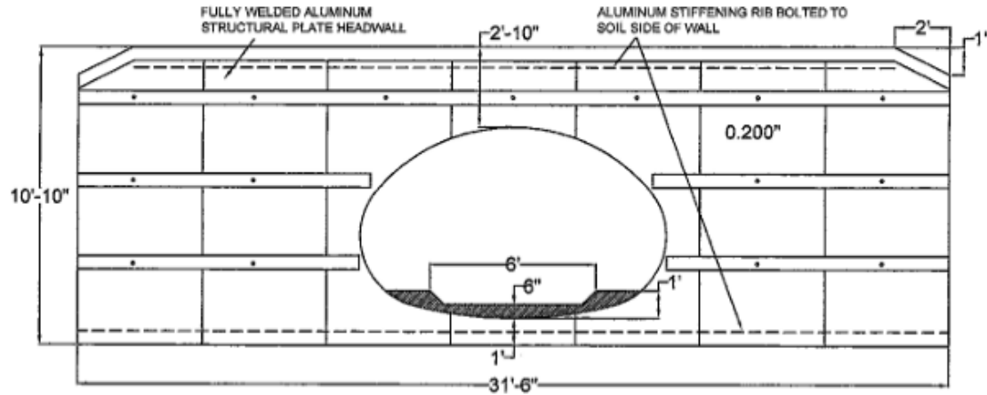
END VIEW- INLET HEADWALL
