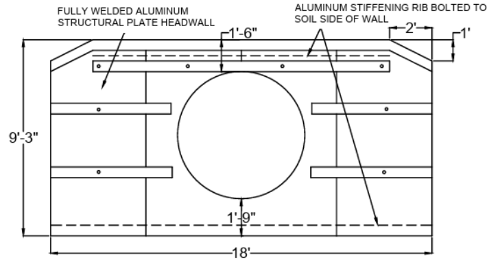
END VIEW- INLET & OUTLET HEADWALL
