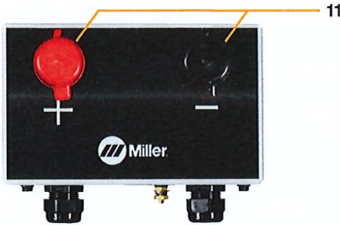
Weld output panel (A60GBW and A60GBHW models only)
