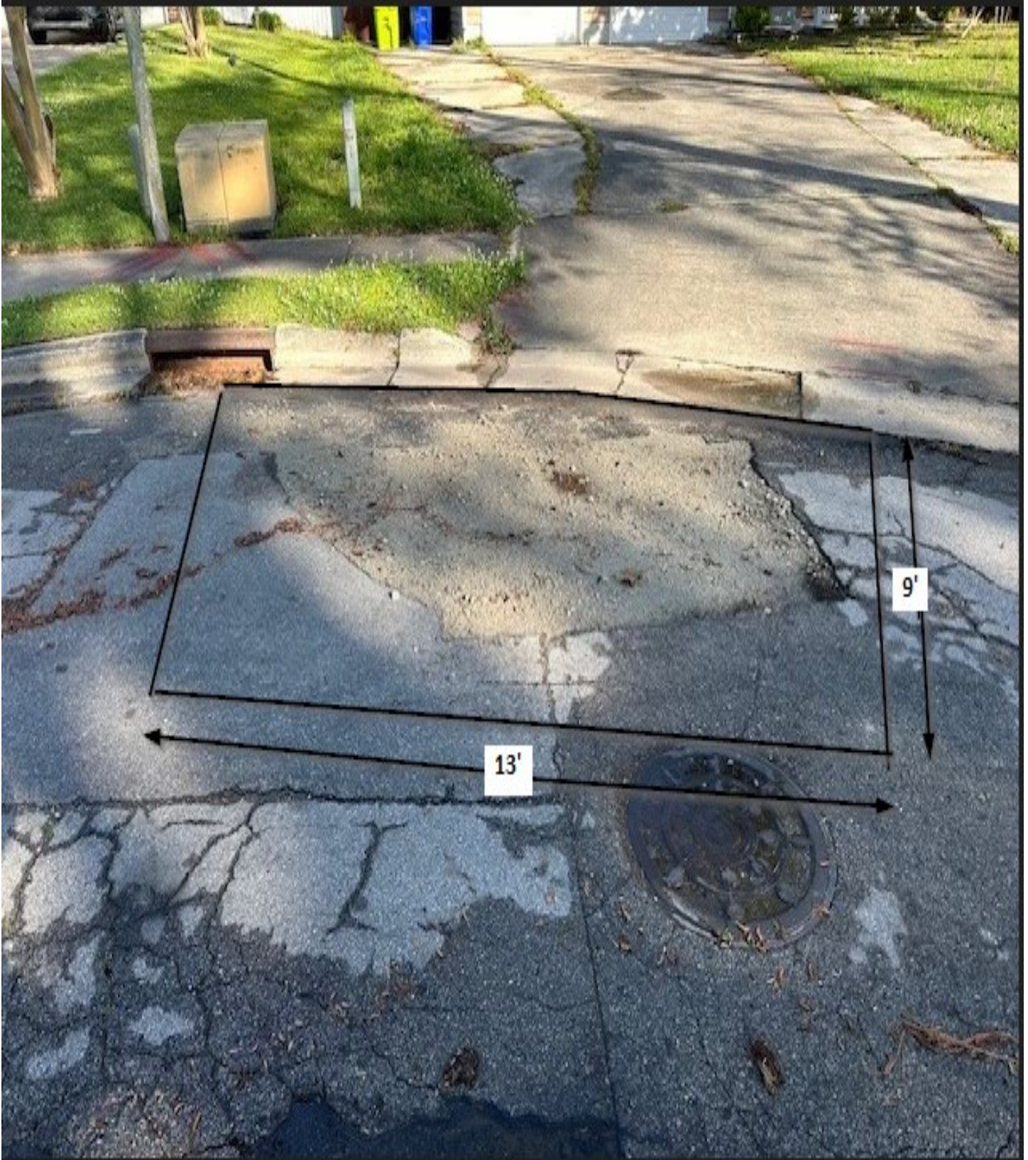
Figure 31: 117 Stonebridge Tr. / Area G / This area shall be cut square before repairing the utility cut. Measurements are approximate.
