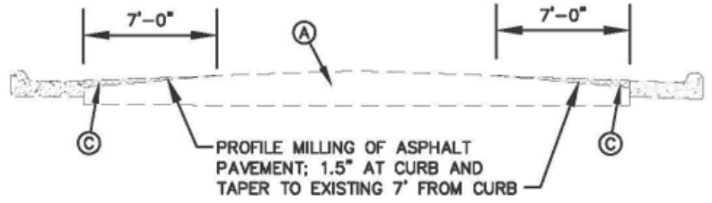
MILLING TYPICAL SECTION #1
