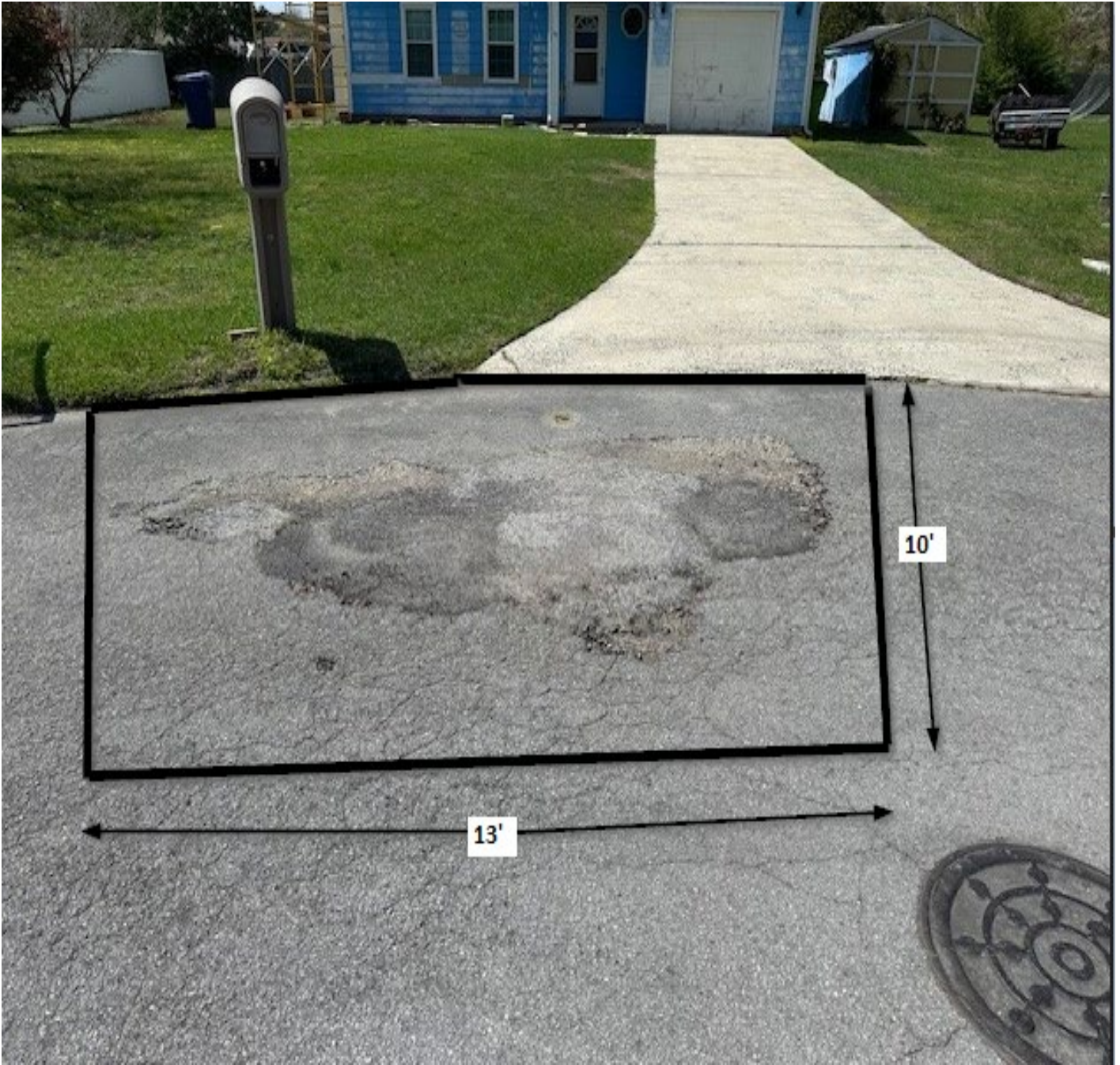
Figure 2: 317 Beechwood Utility Cut / Area A / This area shall be cut square before repairing the utility cut. Measurements are approximate.
