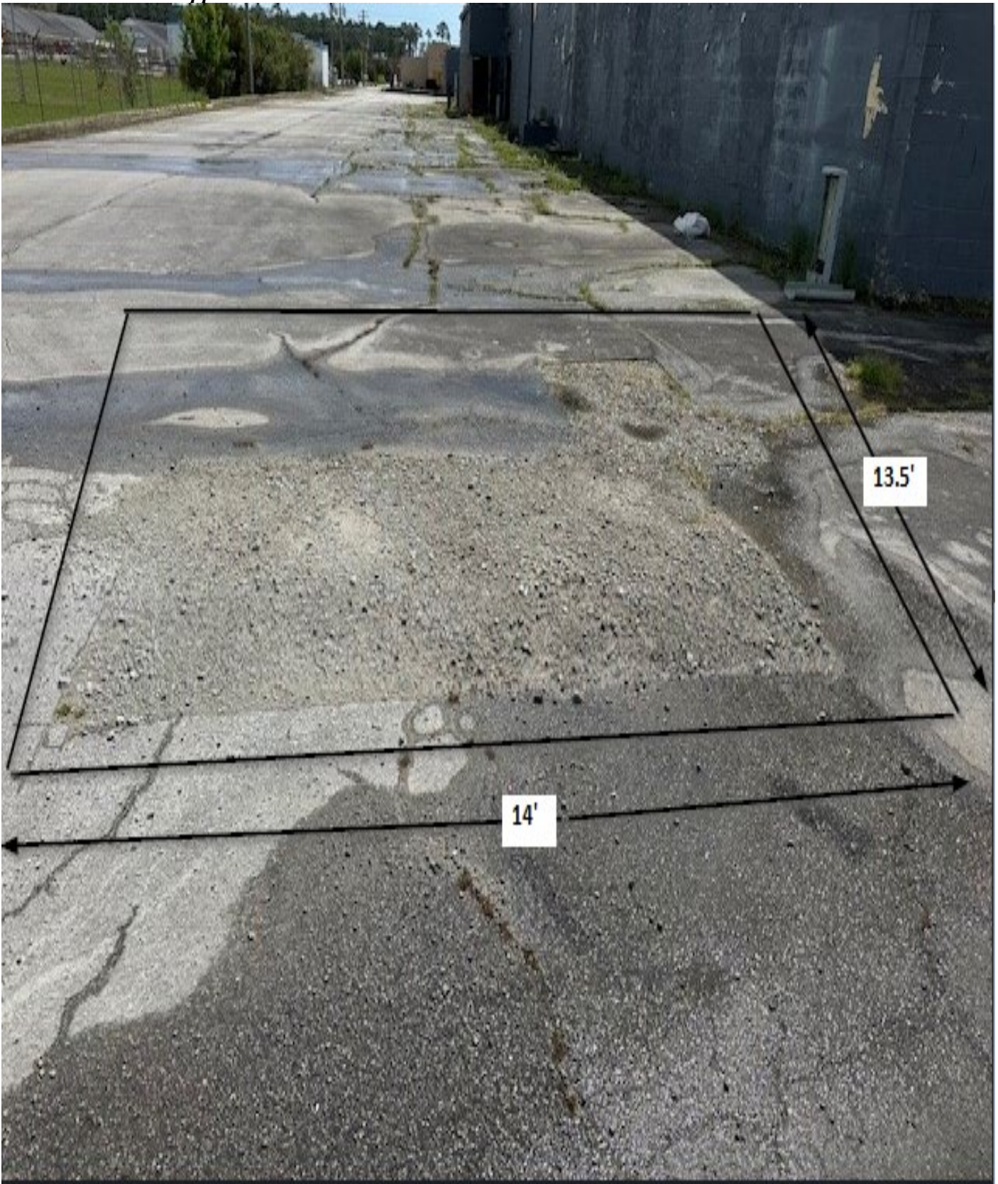
Figure 19: 1313 A E. Main St. / Area A / This area shall be cut square before repairing the utility cut. Measurements are approximate.
