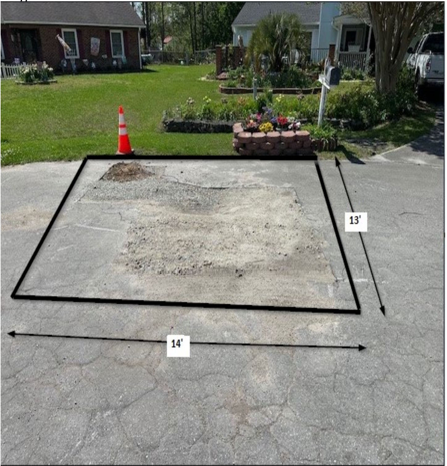
Figure 17: 522 Gene / Area A / This area shall be cut square before repairing the utility cut. Measurements are approximate.
