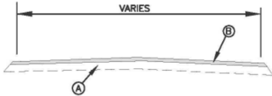
RESURFACING TYPICAL SECTION #1
