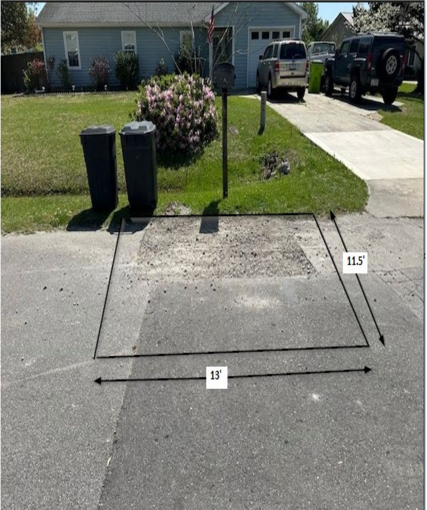
Figure 7: 104 Cindy / Area A / This area shall be cut square before repairing the utility cut. Measurements are approximate.
