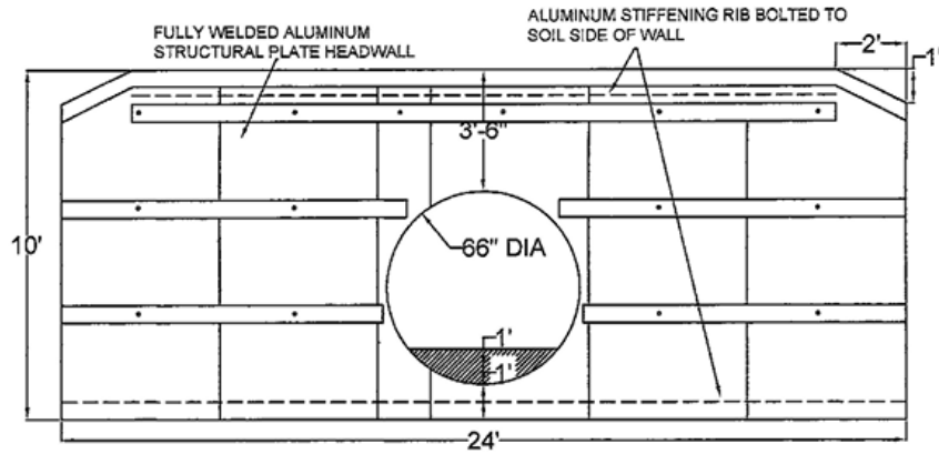
END VIEW- INLET HEADWALL
