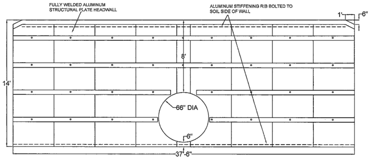
END VIEW- OUTLET HEADWALL
