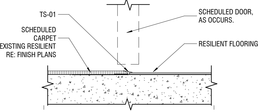
B5 CARPET/EXISTING RESILIENT TO RESILIENT FLOOR 3" = 1'-0"
