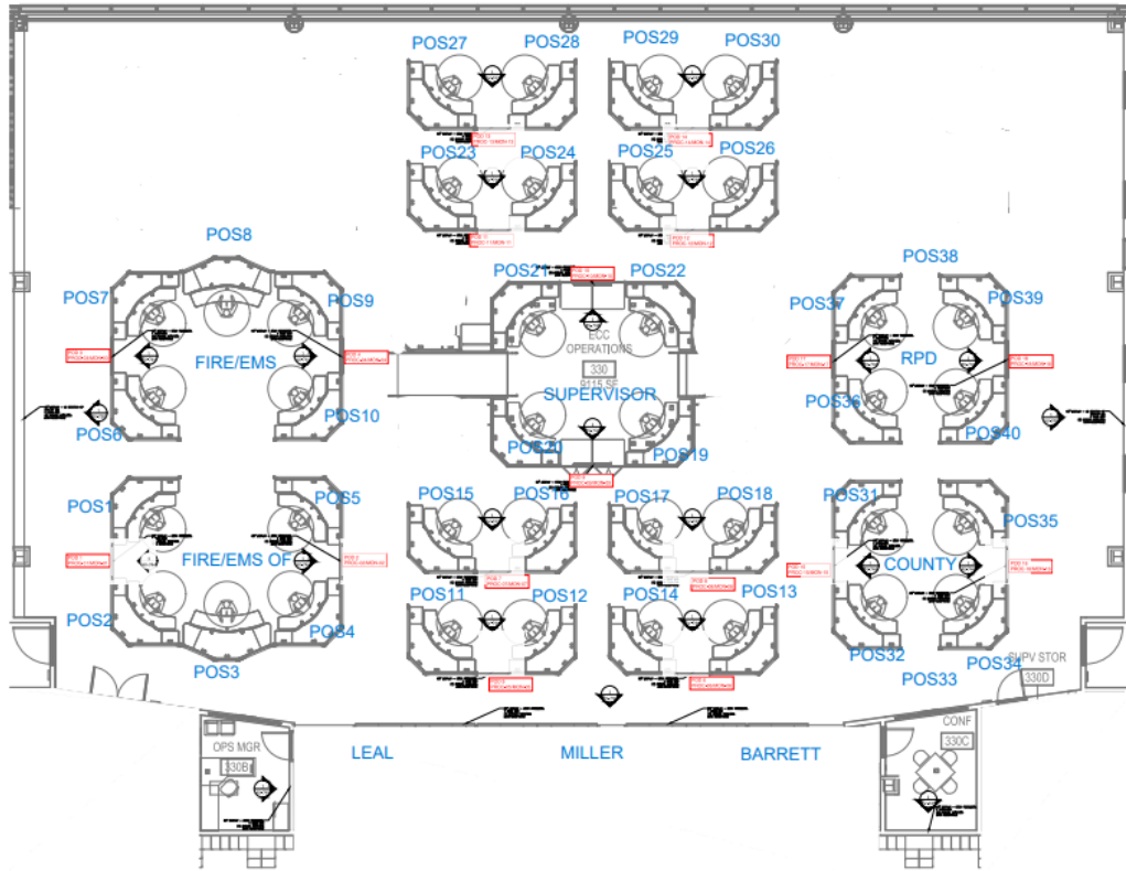
1 FLOOR PLAN - TA103 THIRD FLOOR - OPERATIONS 330, OPS MGR 330B & CONF 330C
