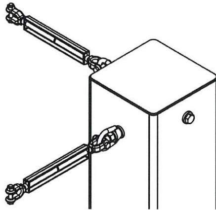
Typical Corner Assembly SEE DETAIL B
