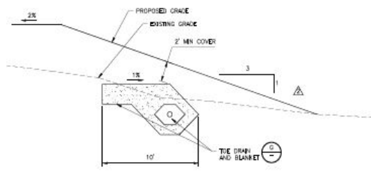
EMBANKMENT WITH TOE DRAIN AND BLANKET
